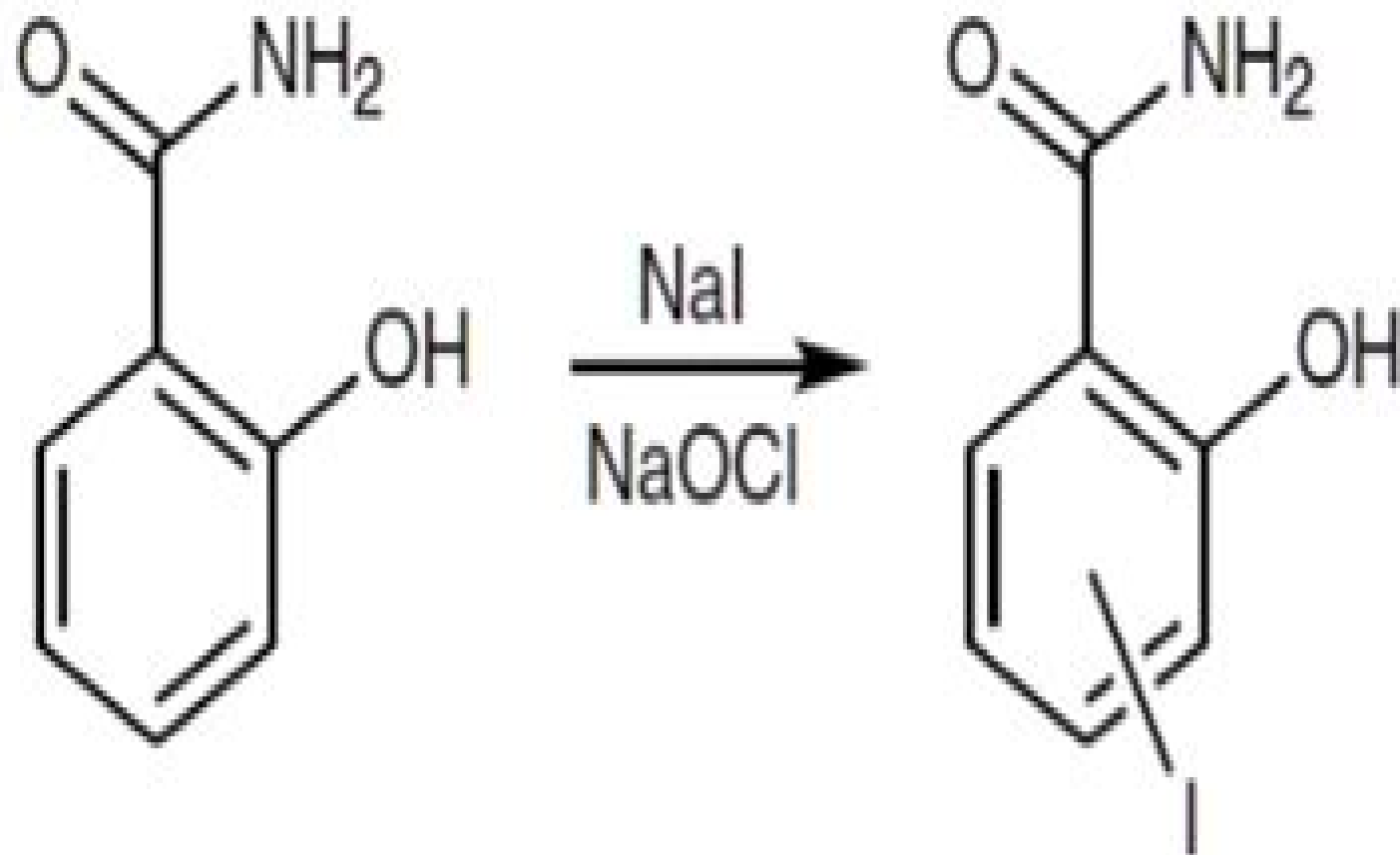
Salicylamide
