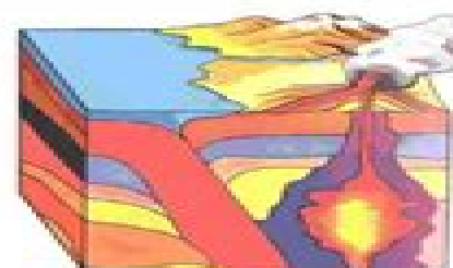
An example of contact metamorphism, where magma changes the type of rock over time
