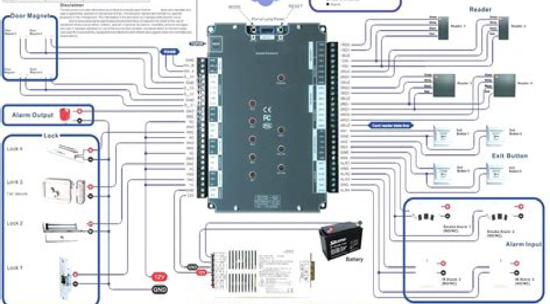
Wiring Diagram of Access Controller
