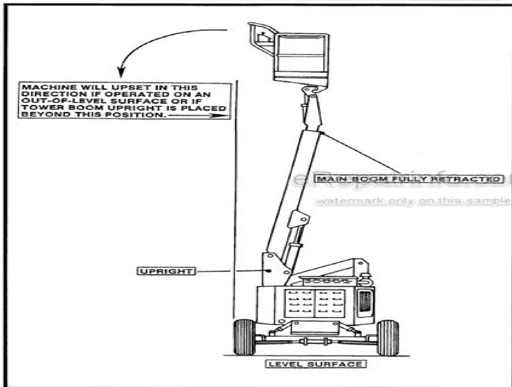
Figure 3-2. Position of Least Backward Stability.
