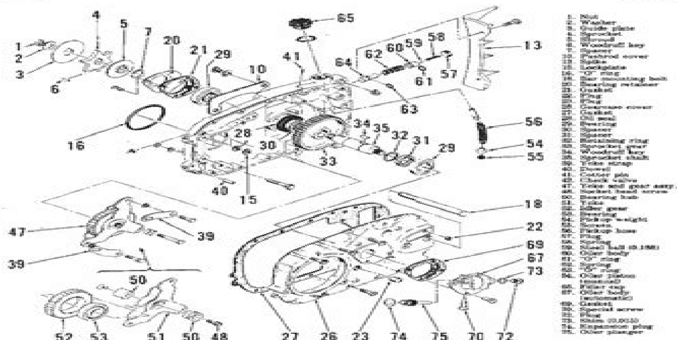
Fig. MC5-24—Exploded view of transmission used on Models 895 and 895C. Input gear is part of clutch drum (38—Fig. MC5-21). Shafts (22) are 5/16" SAE.
