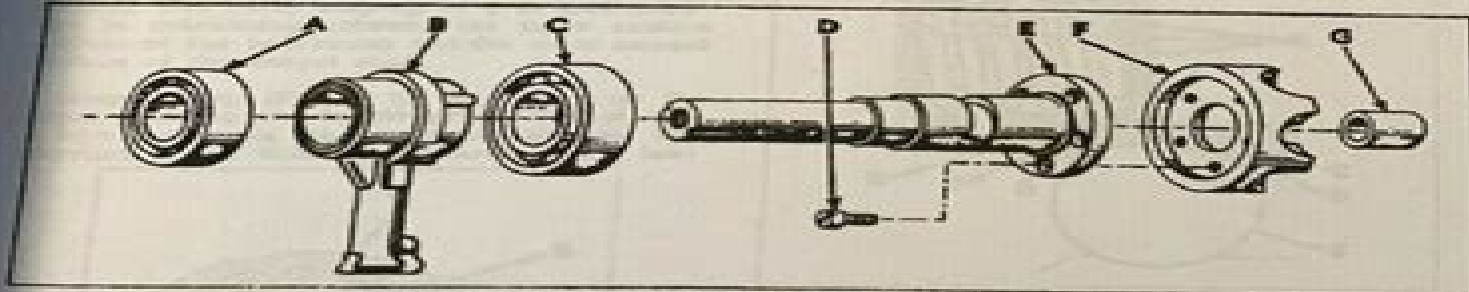
FIG. 4 POWER INPUT SHAFT ASSEMBLY
