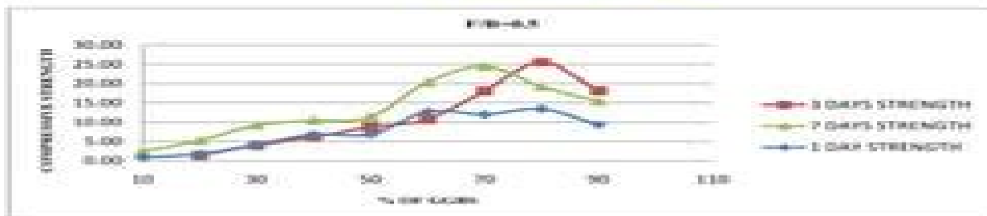
Chart 5, Variation of compressive strength with age at different percentages of COARSE for F15-0.5.
