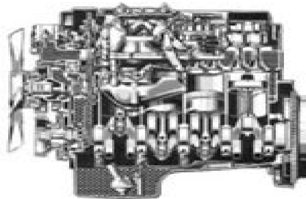
Longitudinal and cross sectional views of engine 102.563
