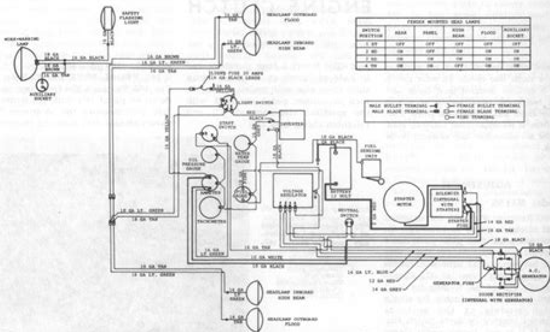
Fig. 194—Wiring diagram for MF135 diesel equipped with alternator. Other late models are similar.
