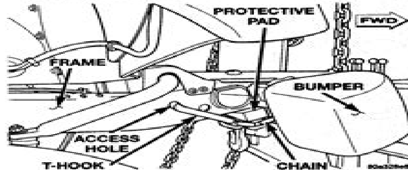
Fig. 3 T-Hook Attachment
