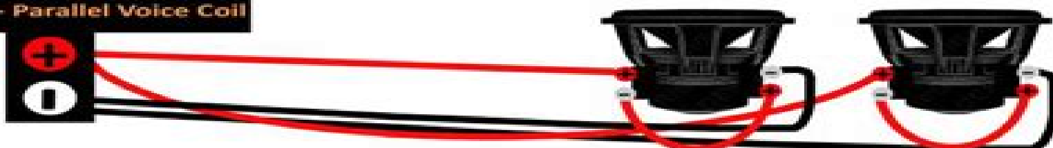
Dual Sub, Series - Parallel Voice Coil
