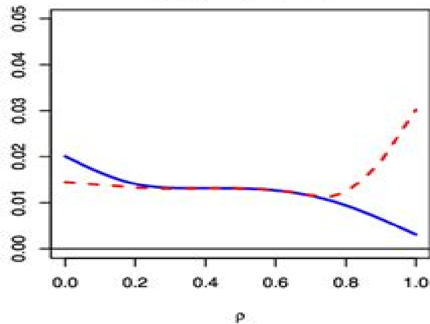
(\pi_0, \gamma) = (0.8, 0.1)
