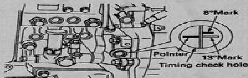
Fig. 26 Timing check hole
