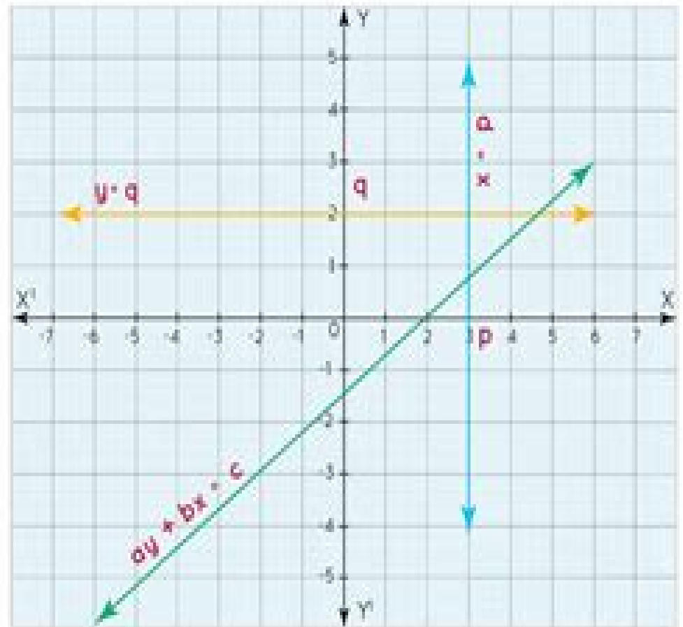
Graphical Representation of Linear Equations
