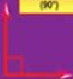
Intersecting Lines
