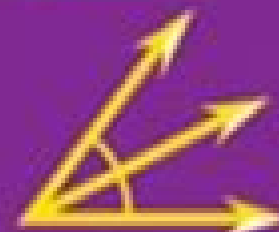
Angle Bisector
