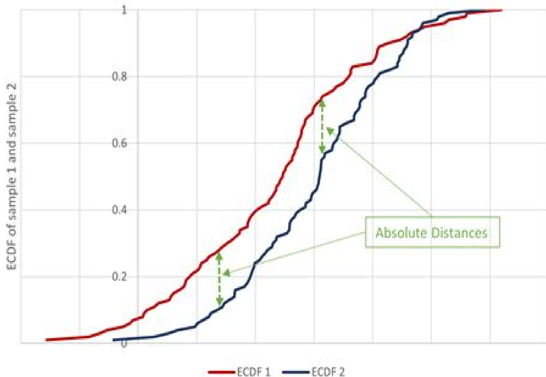
Distributions of both samples
