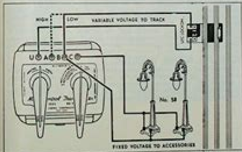
Figure 2—Track and Accessory Connection for "Multi-Control" Transformer
