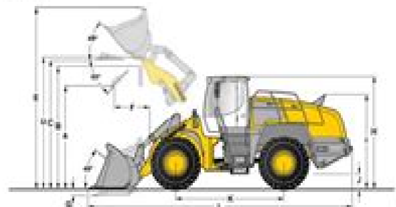
Fig. 8: Complete machine with bucket (industrial lift arms)
