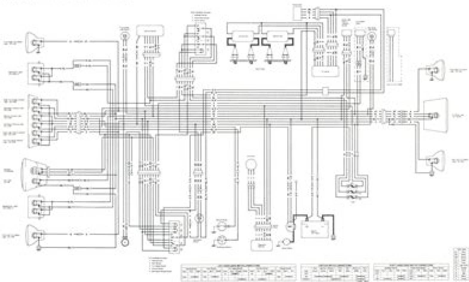
Z650-F4 Wiring Diagram (West German and U.K. models)
