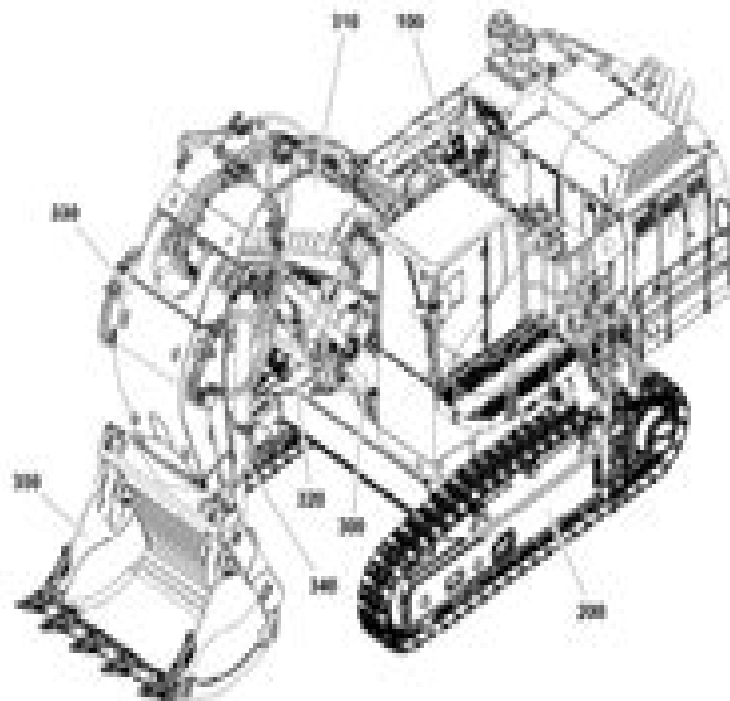
Fig. 1-2 Machine and construction equipment - shovel attachment
