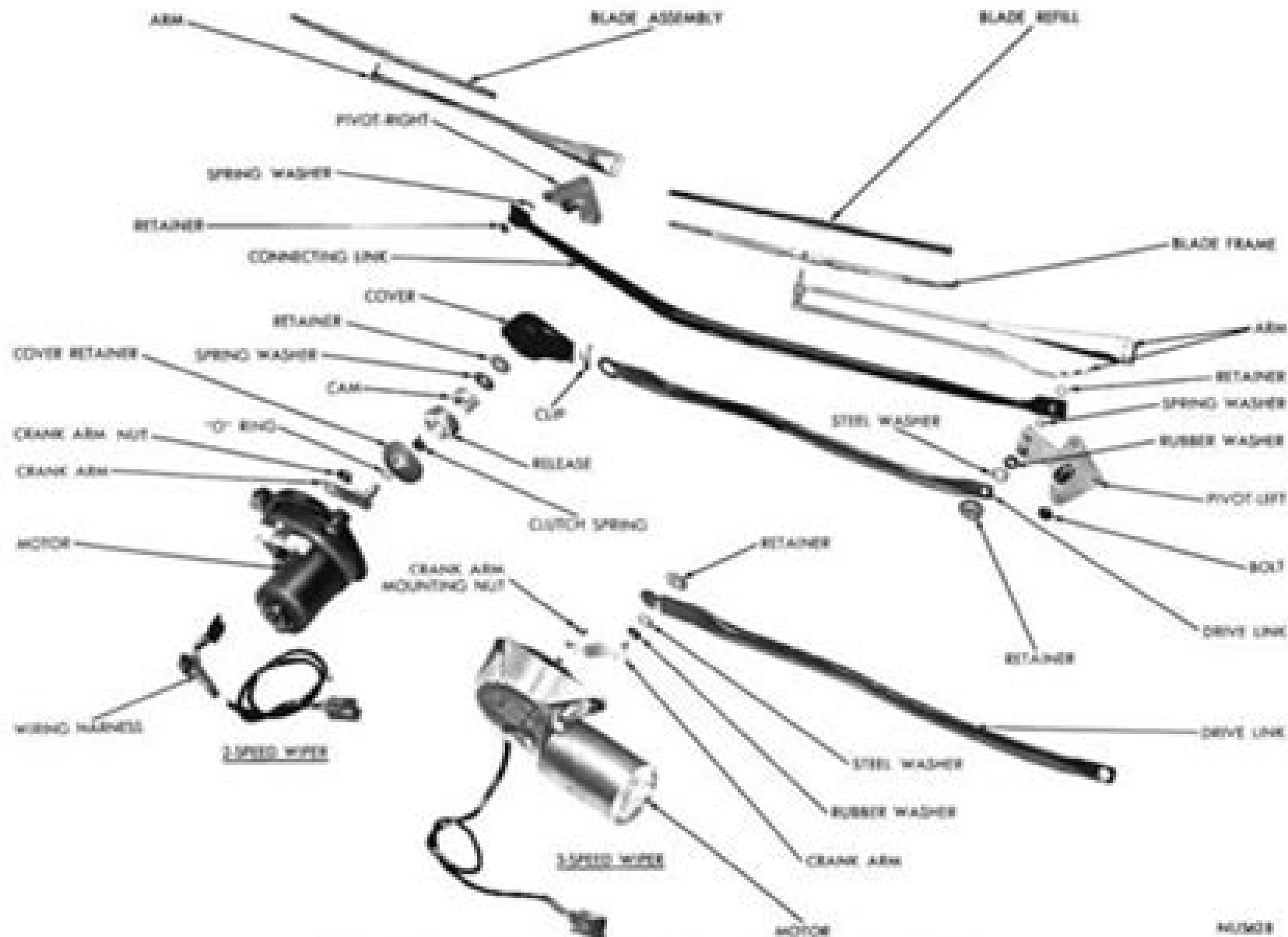
Fig. 14 - Two and Three Speed Wiper Systems (With Concealed Wipers.)
