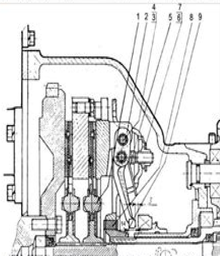
1- damper element; 2- square lever; 3- square lever axle; 4- rollers; 5- support yoke; 6-adjusting nut; 7- backing plate; 8- resilient backing plate element; 9- PTO drive hub.
