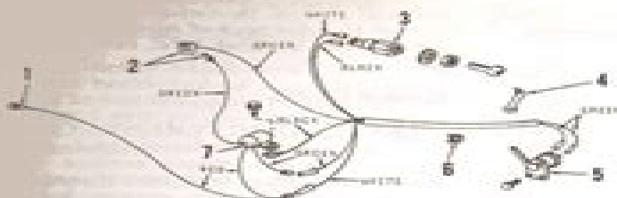
Fig. JD14—Pictorial view of ignition and safety start circuits for Models 55 and 56 with manual start.
