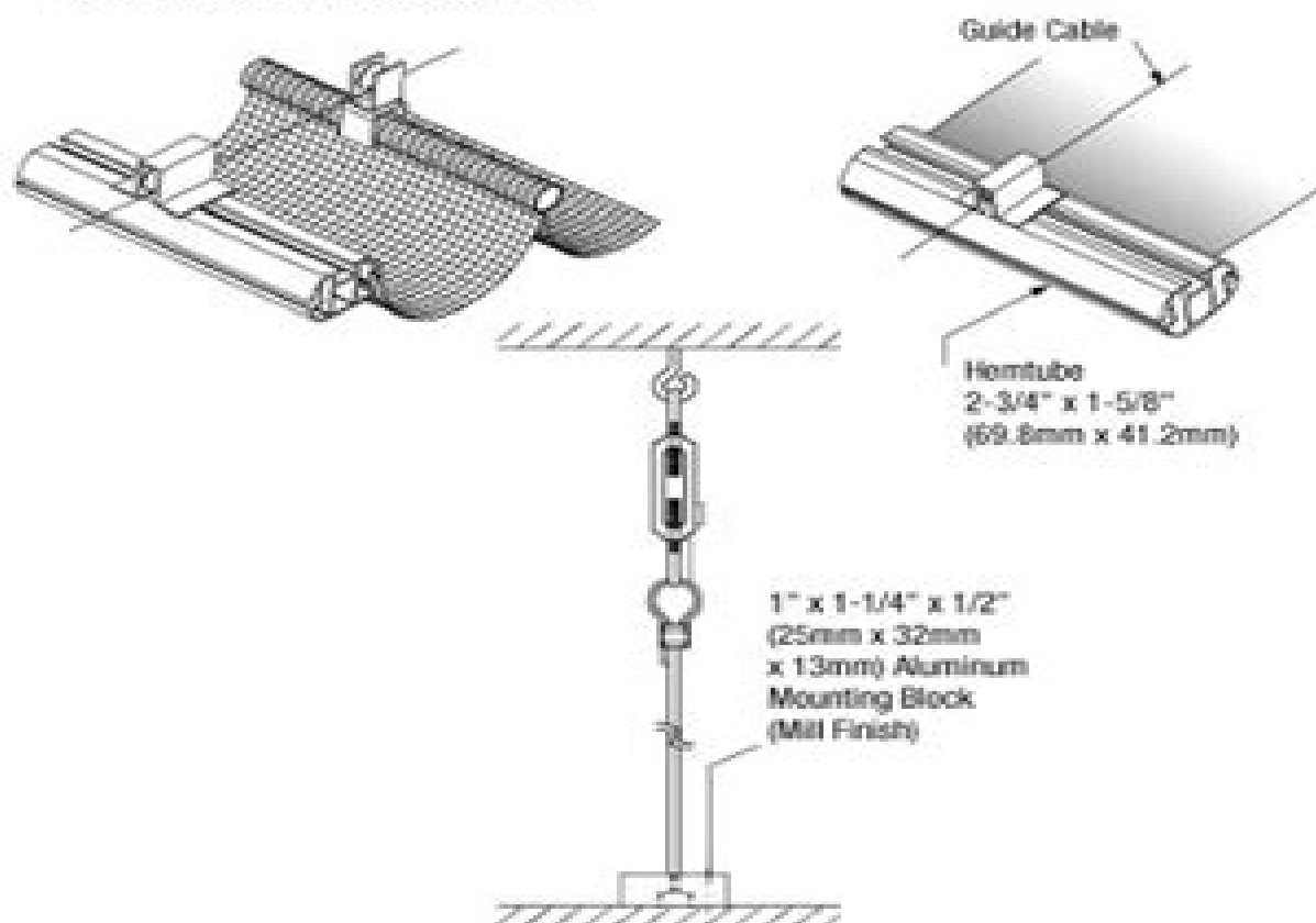
GP Hemtube with Guide Cable Detail
