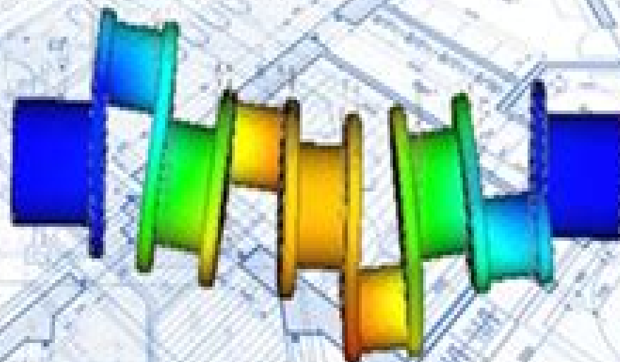
Mode Shape 1 - Frequency 104.6 Hz
