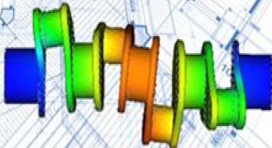
Mode Shape 2 - Frequency 151.7 Hz
