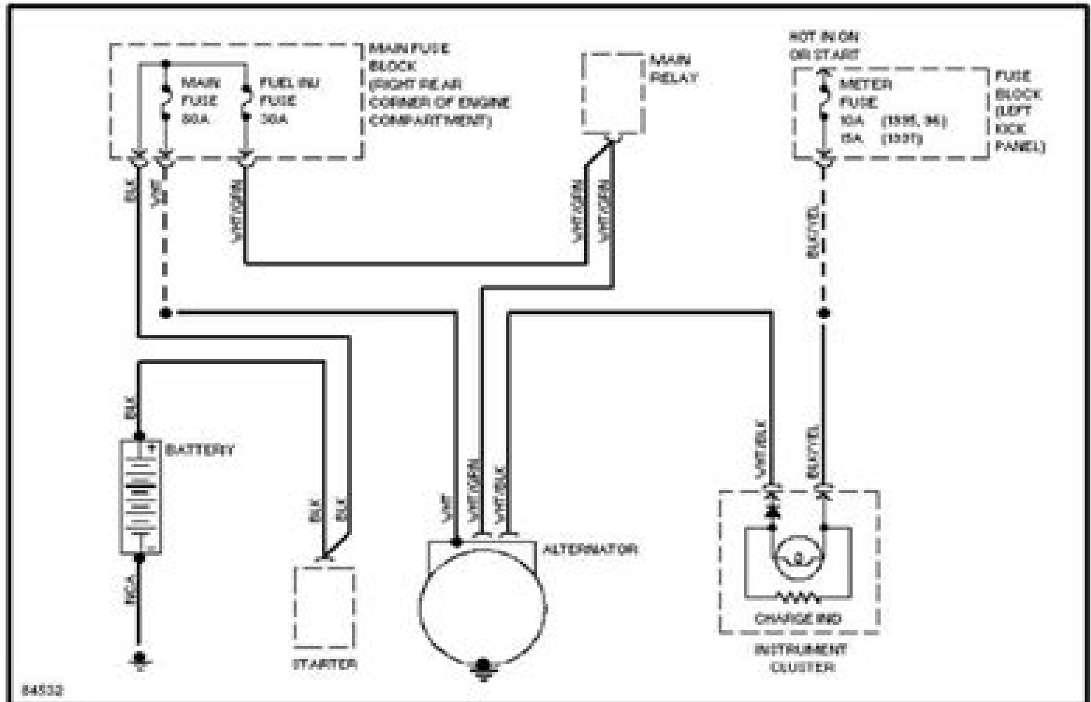
Charging Circuit
