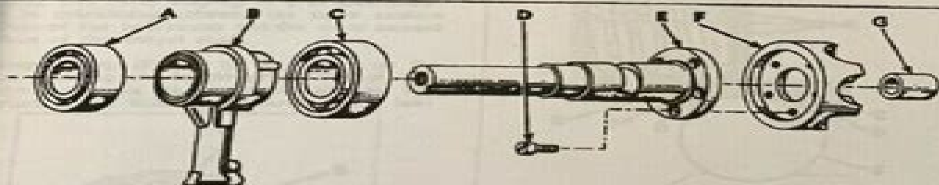
FIG. 4 POWER INPUT SHAFT ASSEMBLY
