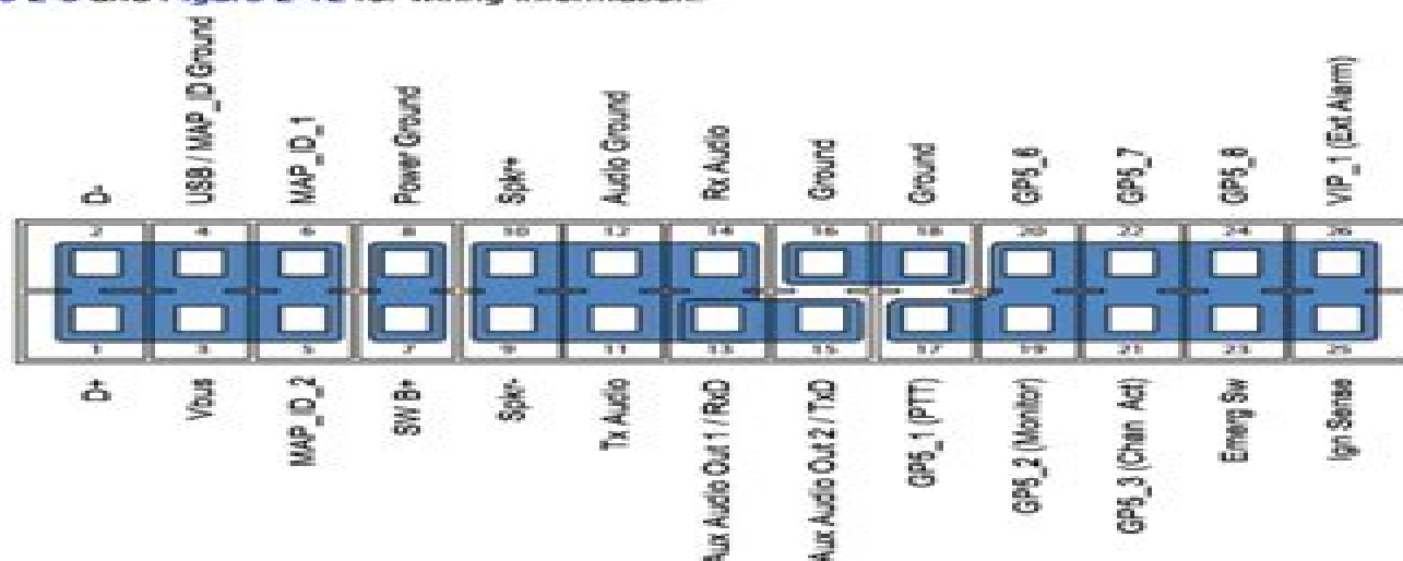
Figure 3-2 Pin Configuration of Rear Accessory Connector (as viewed from the rear of the radio)
