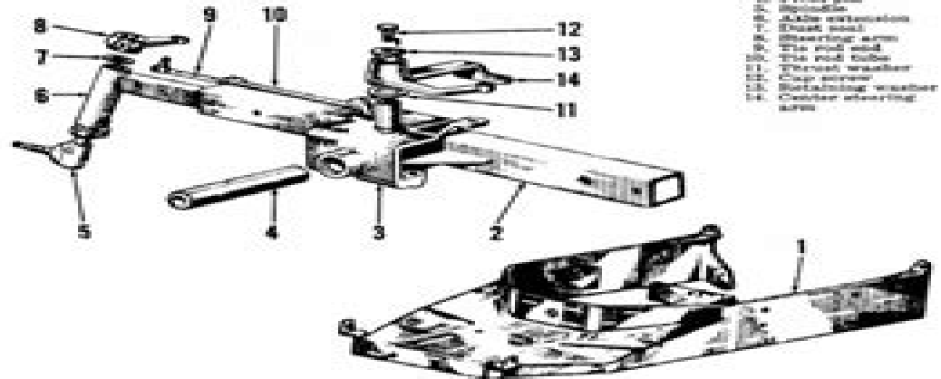
Fig. 1—Exploded view of engine frame, front axle, front support and associated parts used on Model MF25. Axle is similar on Model MF10, but cast from support bolts to cast iron oil pan and engine frame is not used. Refer to Fig. 2.
