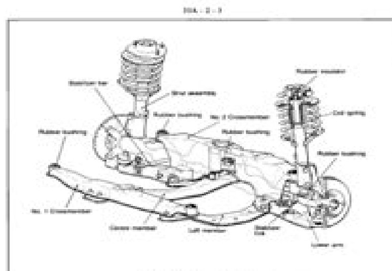
Fig. 1-1 Front suspension components
