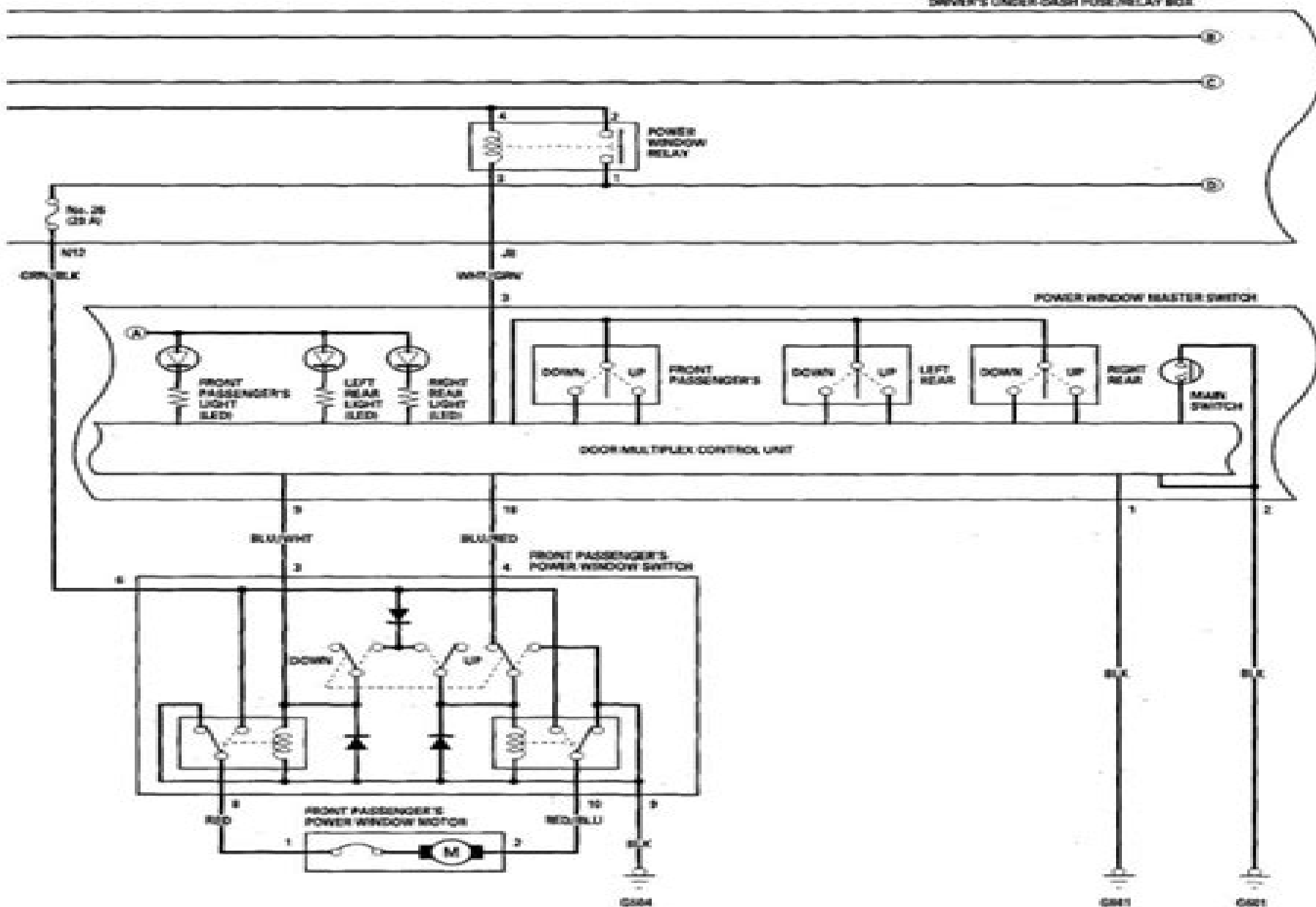
Fig. 5: Power Windows - Circuit Diagram (2 Of 3) Courtesy of AMERICAN HONDA MOTOR CO., INC.
