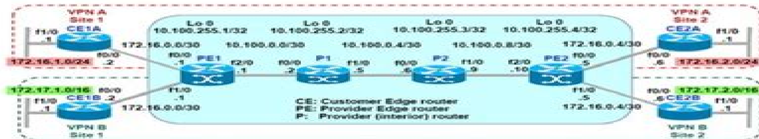
Figure 1. Network configuration for experiments with MPLS-based VPNs.
