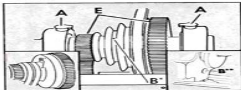
HEADSTOCK AND BACK GEARS
