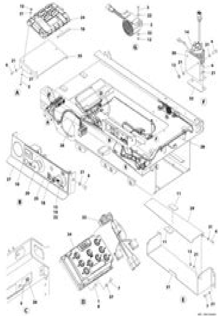
FIGURE 3-2. ELECTRICAL COMPONENTS INSTALLATION (WITHOUT LUG)
