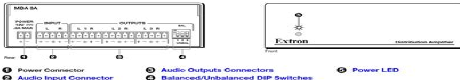
Figure 1. MDA 3A Rear and Front Panels
