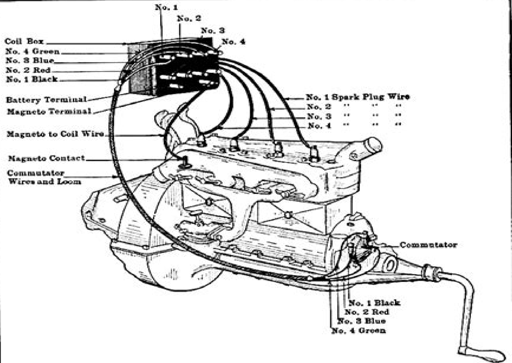
Fig. 16.—View of Ford Power Plant Showing Main Parts of the Ford Ignition System. Note Location of Timer and Induction Coil Box.
