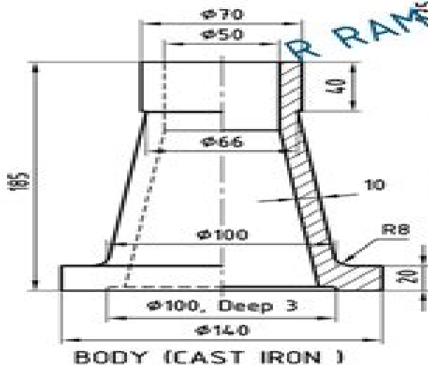
BODY (CAST IRON)
