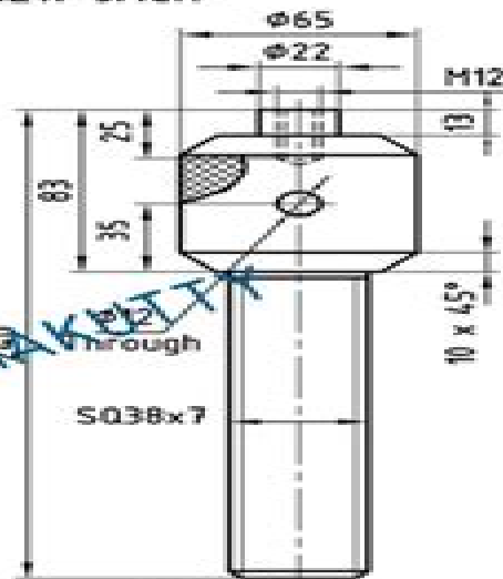
SCREW SPINDLE (MILD STEEL)
