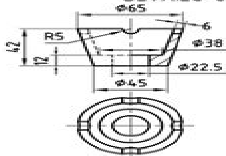
CUP (CAST STEEL)
