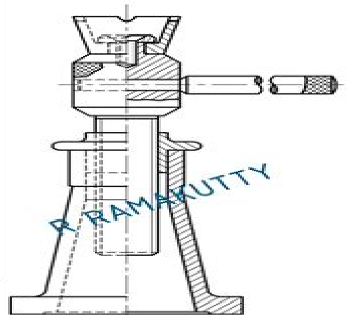
Half Sectional Front View
