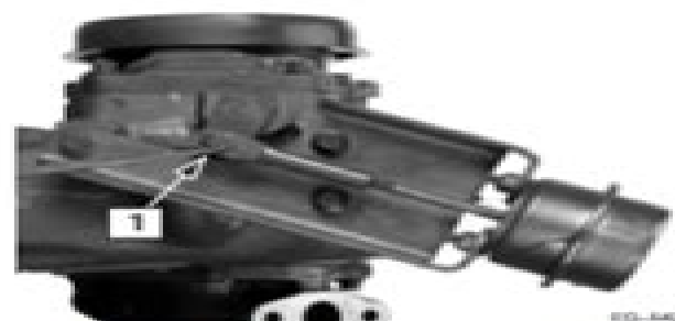
Figure 2.12 Remove Retaining Clip 1. Retaining Clip
