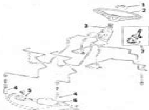
Fig. 3—Schematic view showing general layout of component parts of typical power steering system on International tractors. Ross hand pump and steering valve (7) is used on Models 434, 464, 574 and 574. Denso pump and steering valve (7) is used on Models 484 and 584.
