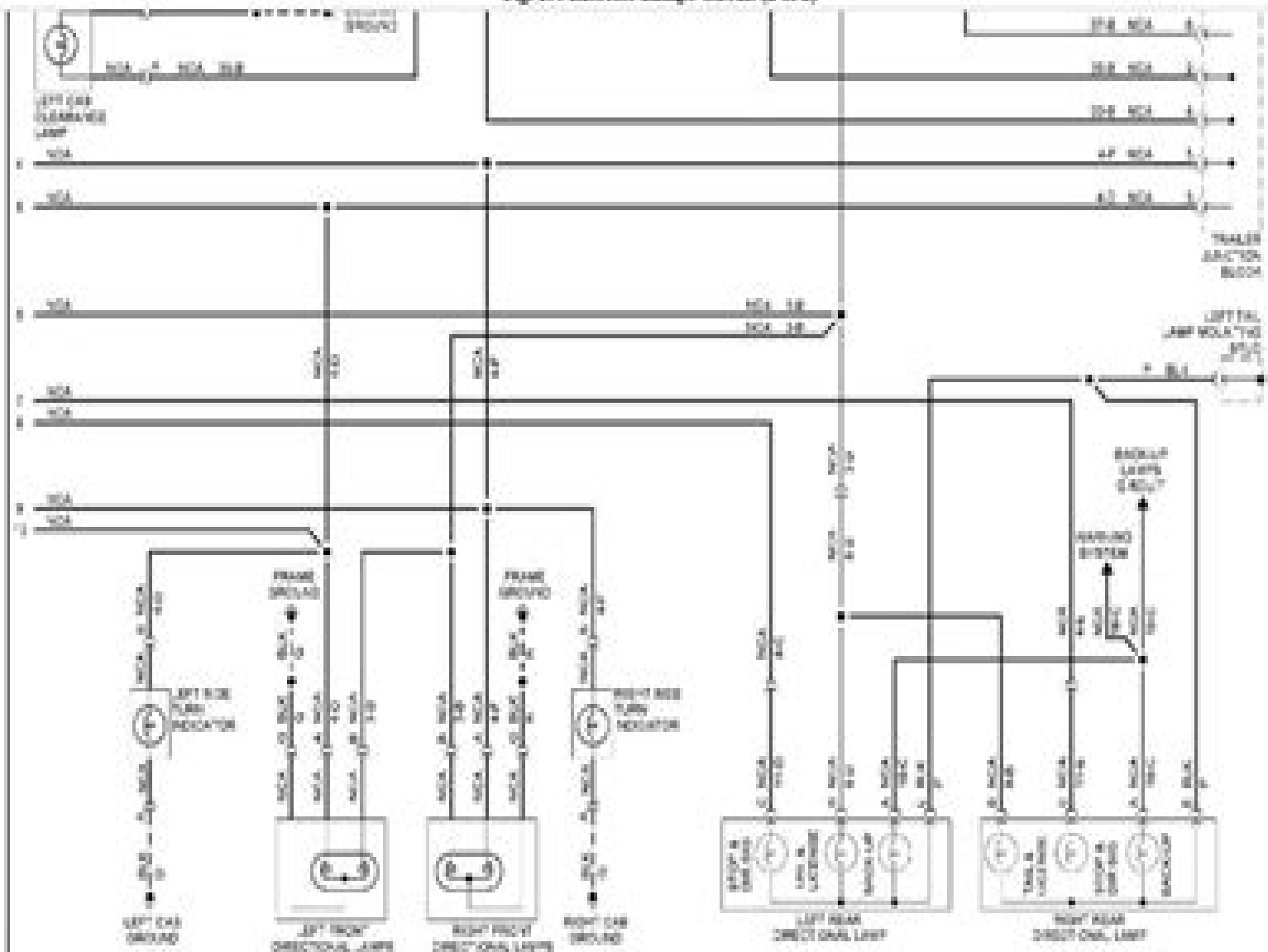
1995 Mack CH Series - CH413 Fig. 19: Exterior Lamps Circuit (2 of 2)
