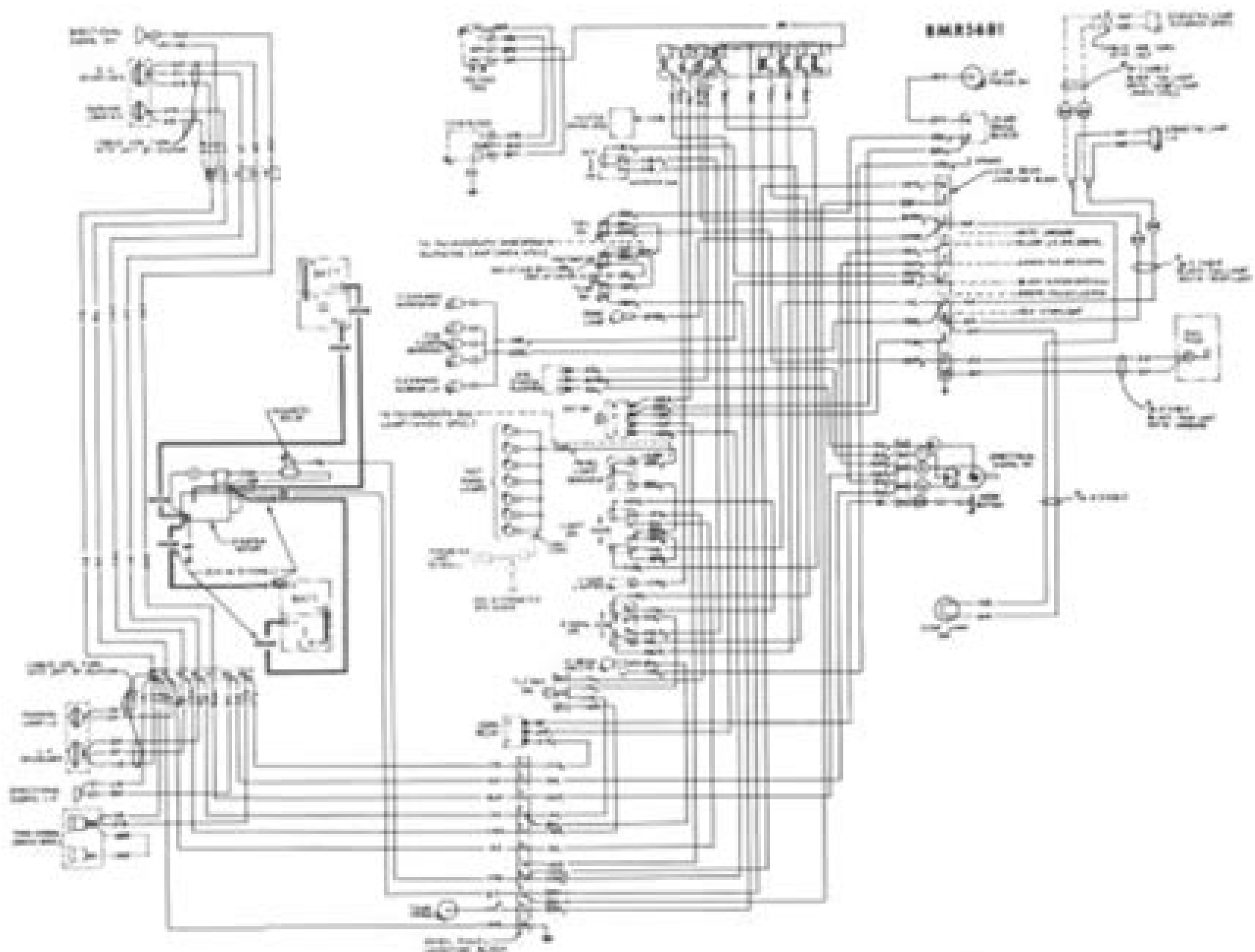
Figure 15-8. Wiring Schematic "R" and "U" Models 12 Volt Parallel Starting
