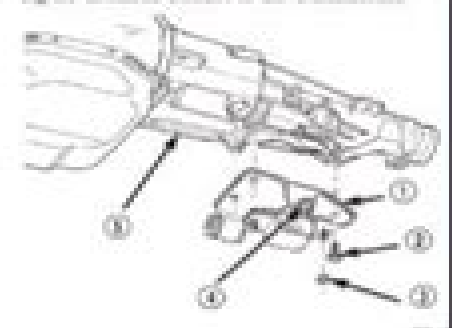
Fig. 49 Engine Rear Mount-4x4 Automatic Transmission 1 - ENGINE REAR MOUNT 2 - ENGINE 3 - BOLT 4 - NUT
