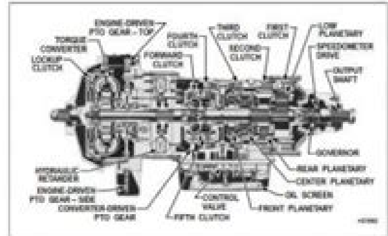
Figure 3. CLBT 750/754 Remote Mount—Cross Section
