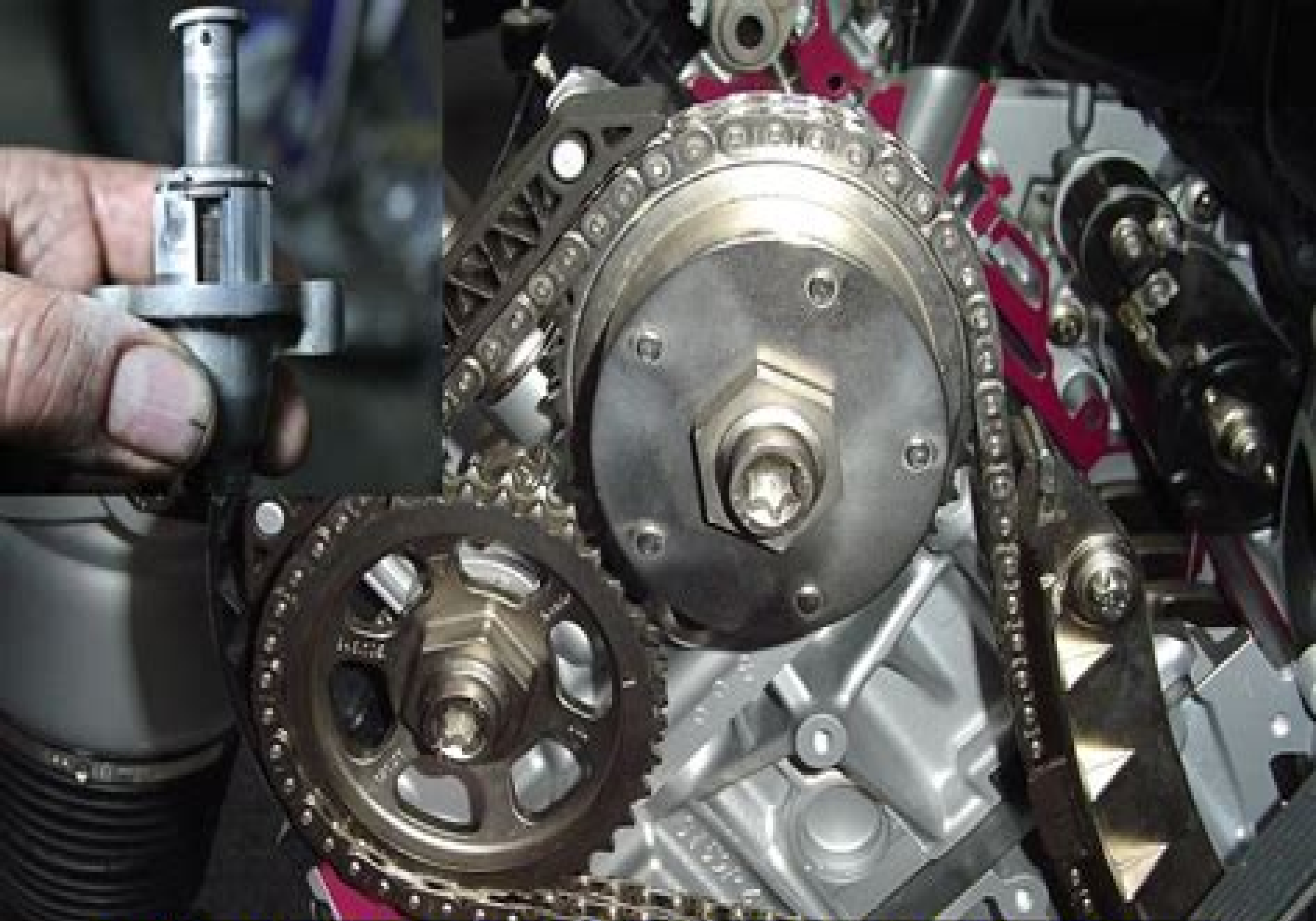
Adjusting Automatic Cam Chain Tensioner
