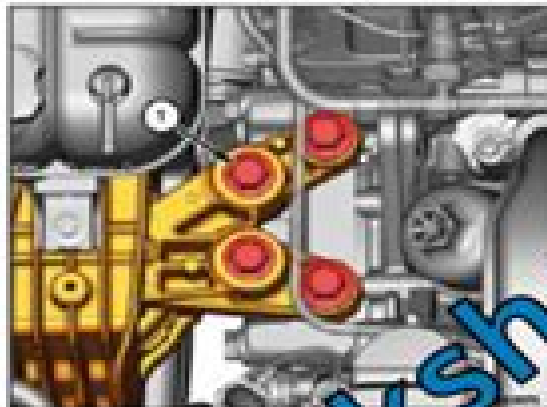
44. Remove the four bolts (1) from the LH engine (transmission) mount bracket.
