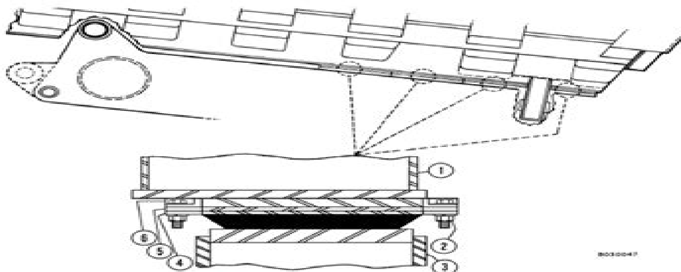
FIGURE 8-9. BODY PAD INSTALLATION
