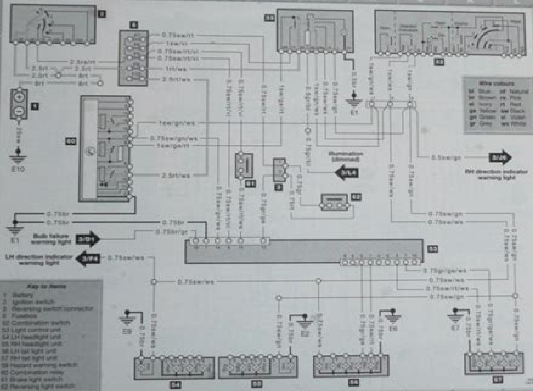
Diagram 5 : Exterior lighting continued - direction indicators, hazard warning, stop and reversing lights
