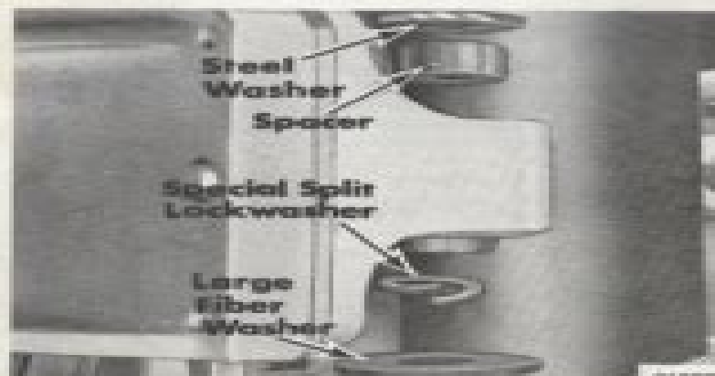
Figure 1. Engine Mounting Bracket Parts
