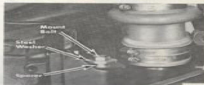
Figure 2. Exhaust Tube and Mounting Bolt Installed
