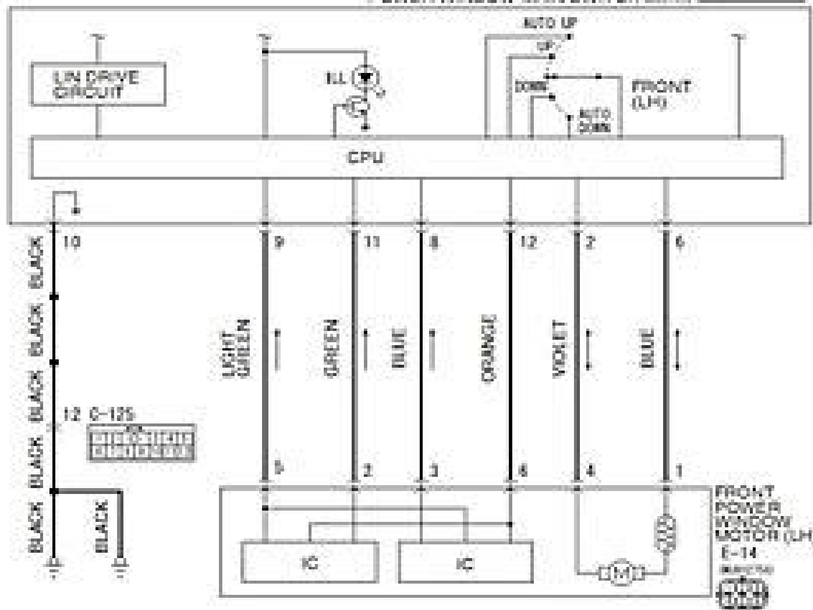
POWER WINDOW MAIN SWITCH
