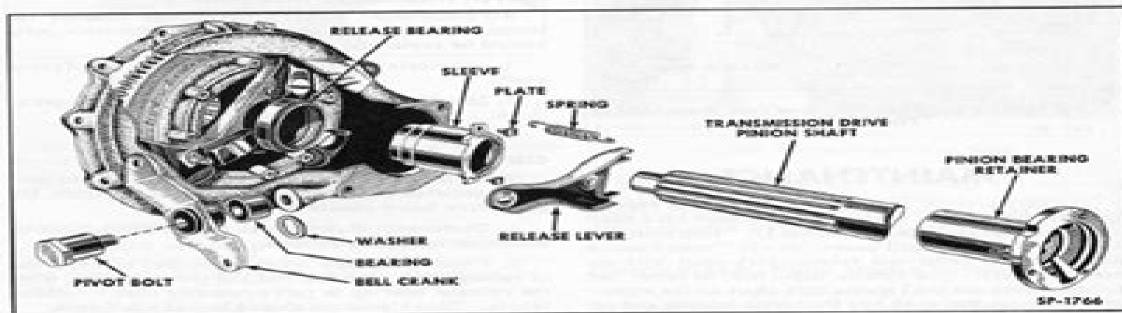
Fig. 103—Typical Clutch Installation—Exploded View
